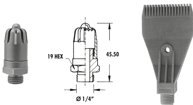
Tipi - SIL210-SIL300 - Types
